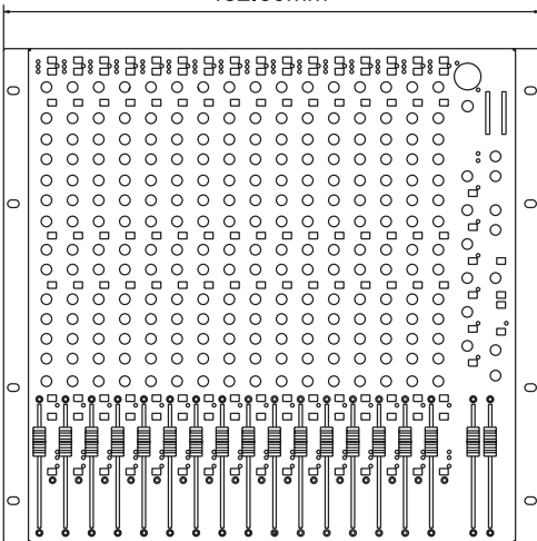
Top View 482.60mm
